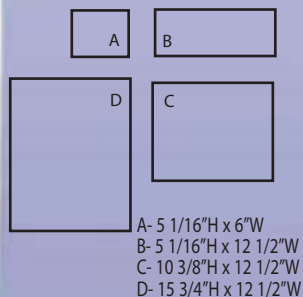
AVAILABLE DOOR SIZES
